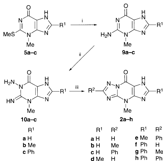
Scheme 2 Reagents and conditions: i, liq. NH 3 , 150 °C, 50 kg cm -2 , 2 d; ii, H 2 NOSO 3 H, 1M NaOH, room temp., 4 d; iii, R 2 C(OEt) 3 , reflux, 10–15 h, or R 2 -CHO, DMF, DEAD, 50–100 °C, 10 h
